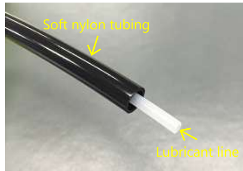
Dual tube [2 channel system] (Soft nylon air tubing)
