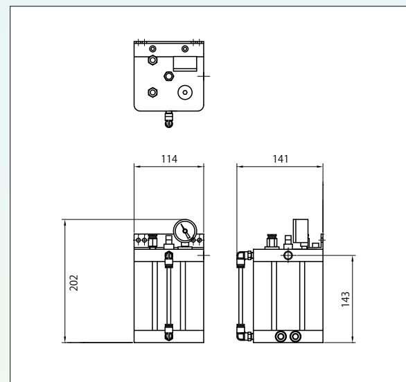
Model BK
