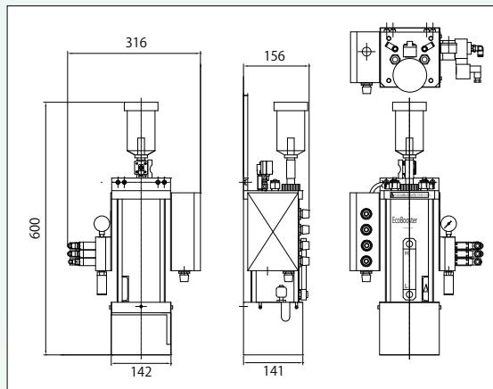
Model EB7EP
