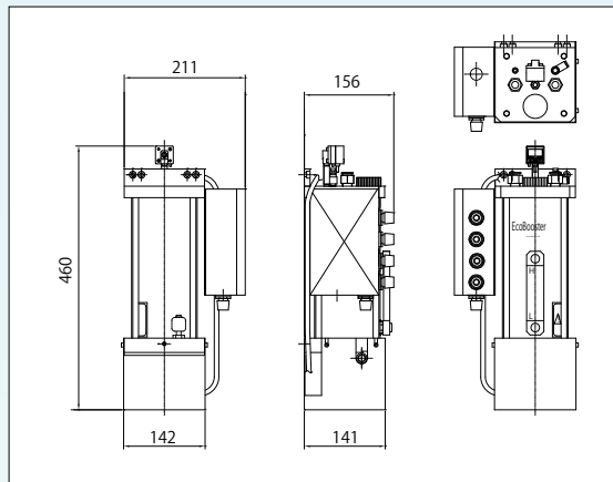
Model EB3EP
